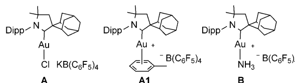
Scheme 1. CAAC–gold(I) catalysts A , A1 , and B (Dipp = 2,6-diisopropylphenyl).
